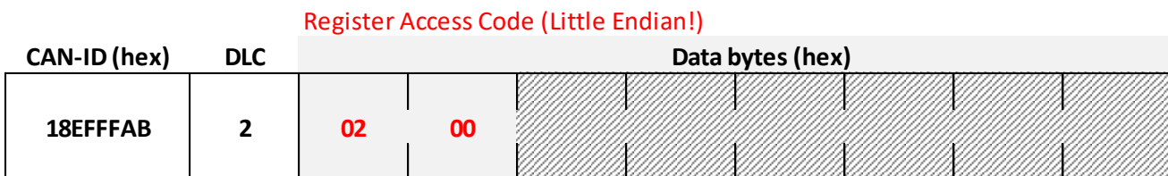
Exemplary access for reading a value from register 0x0002
