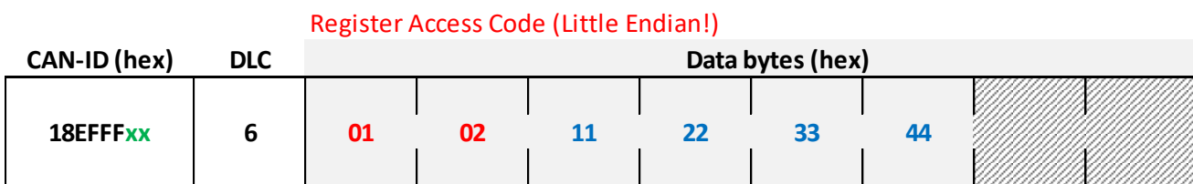
xx stands for the transducer's address Read Value 0x44332211 (in this case int32; Little Endian)
