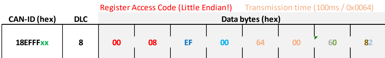
xx stands for the transducer's address PDU Format Priority Autostart PDU Specific Data Page DLC
