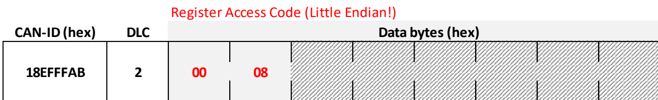
Read PGN settings
