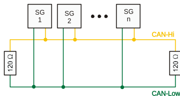
Figure 1: Linear CAN bus topology with terminating resistors [1]
